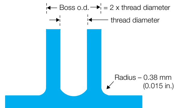
Figure 70: Boss design for self-tapping screws
