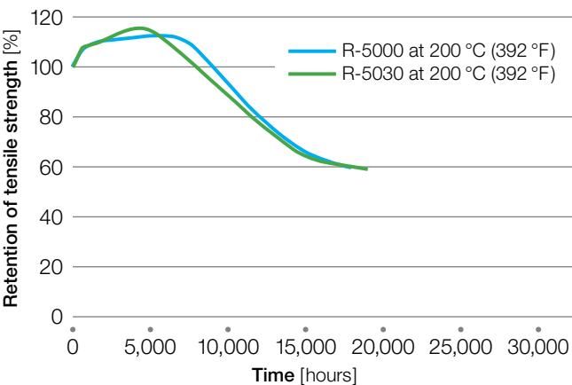
Figure 40: Thermal aging of Radel® PPSU
