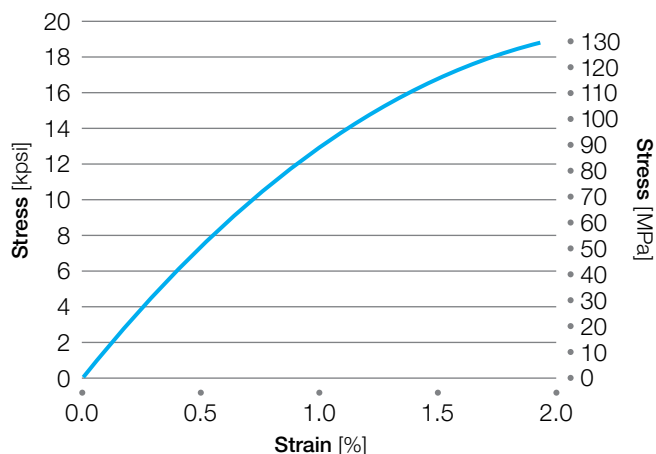
Figure 13: Veradel® AG-330 stress-strain curve to break
