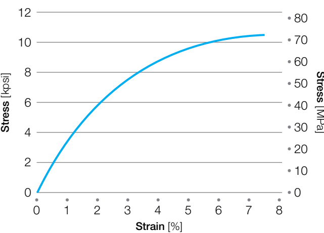
Figure 11: Acudel® 22000 stress-strain curve to yield
