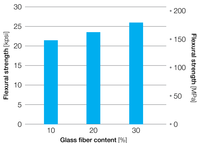
Figure 17: Flexural strength of glass-filled Veradel® PESU
