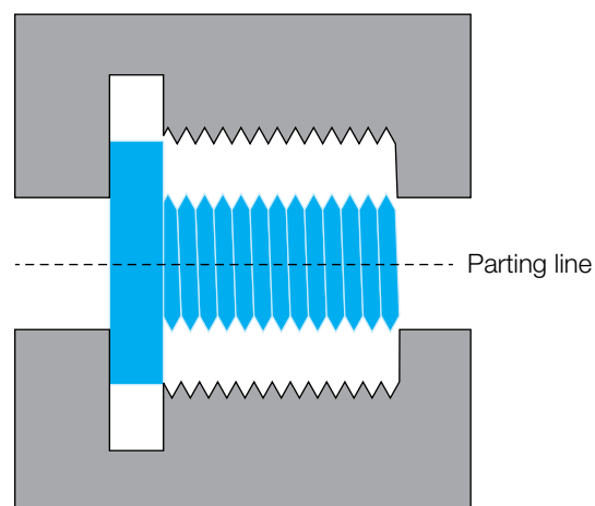
Figure 69: External threads
