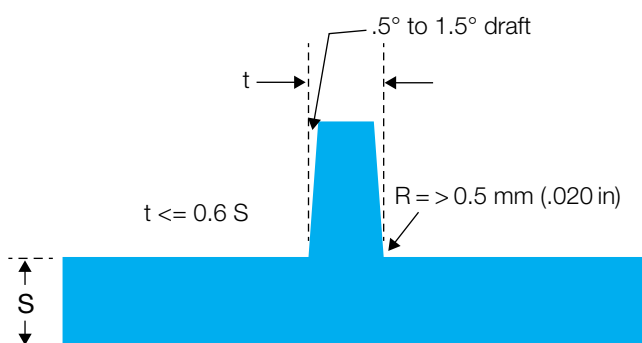
Figure 50: Recommended rib design
