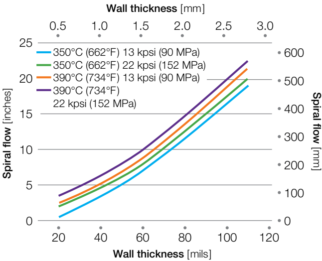
Figure 62: Spiral flow of Veradel® A-301
