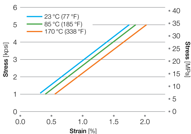
Figure 30: Isochronous stress-strain curve Radel® R-5000 at 100 hours
