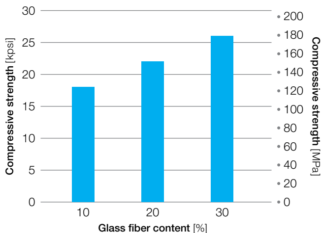
Figure 19: Compressive strength of glass-filled Veradel® PESU
