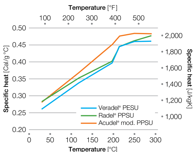
Figure 36: Specific heat
