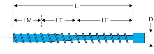
Figure 60: Screw design for injection molding
