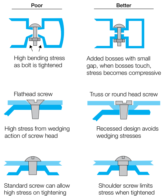
Figure 67: Designing for mechanical fasteners
