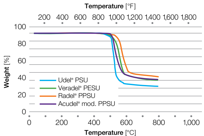
Figure 37: Thermogravimetric analysis in nitrogen
