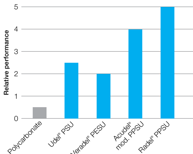
Figure 4: Hydrolytic stability of sulfone polymers
