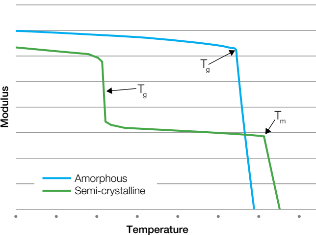
Figure 32: Typical change in modulus with temperature
