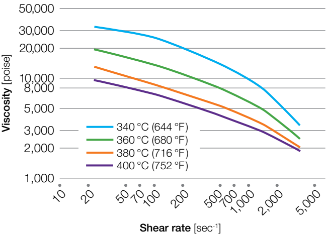
Figure 58: Rheology of Radel® R-5000 resin
