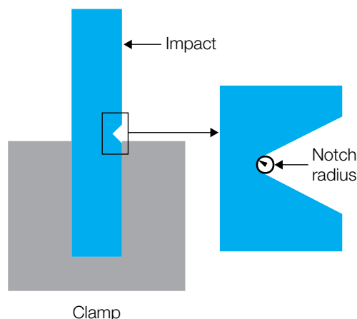
Figure 22: Izod impact test apparatus
