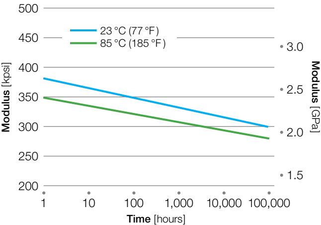
Figure 27: Creep modulus Veradel® A-201 at 20.7 MPa (3,000 psi)
