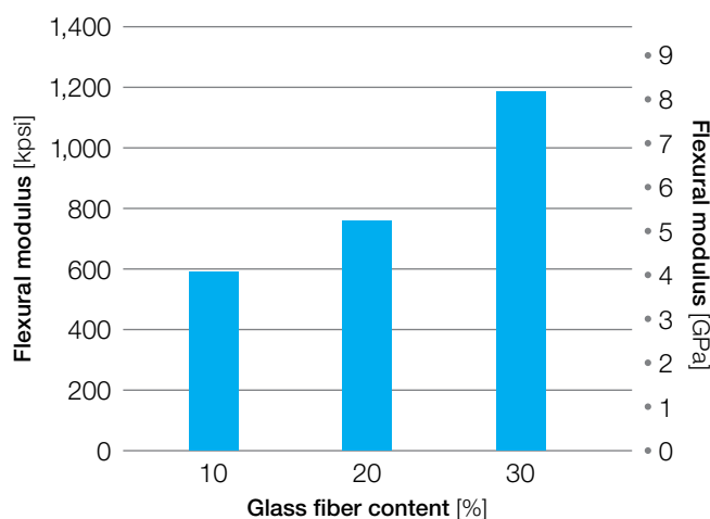
Figure 18: Flexural modulus of glass-filled Veradel® PESU
