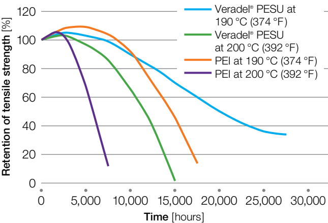
Figure 39: Thermal aging of Veradel® PESU and PEI
