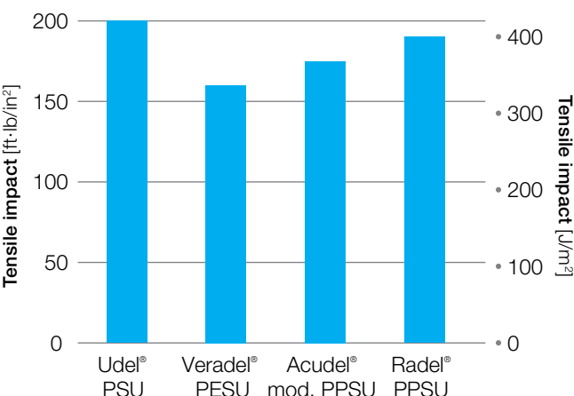
Figure 25: Tensile impact strength of neat resins
