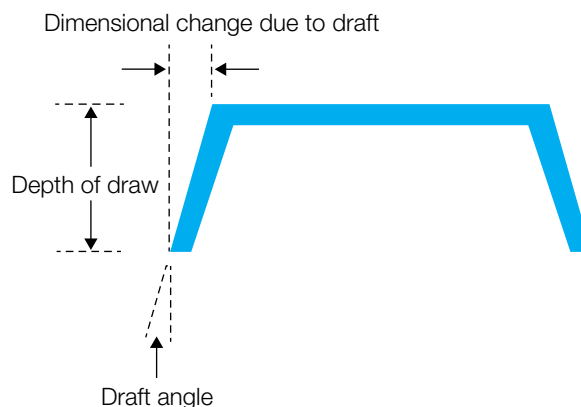
Figure 49: Designing for mold release
