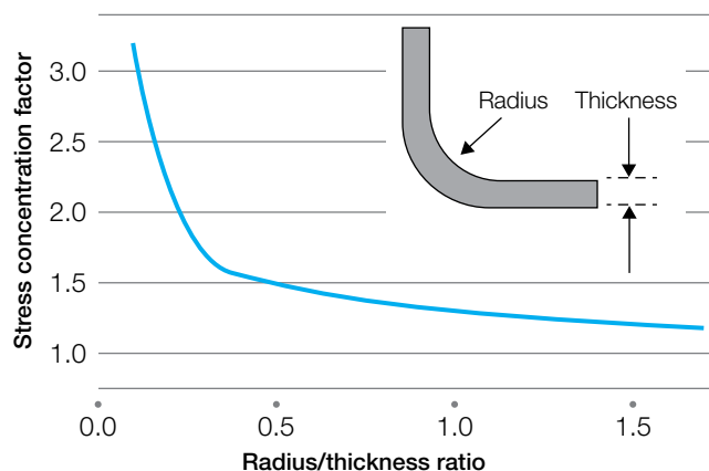
Figure 47: Stress concentration factor at inside corners
