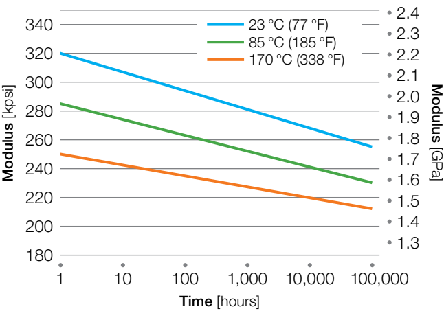
Figure 28: Creep modulus Radel® R-5000 at 20.7 MPa (3,000 psi)
