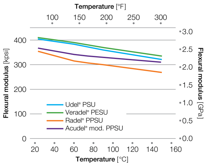
Figure 33: Flexural modulus vs. temperature of neat resins
