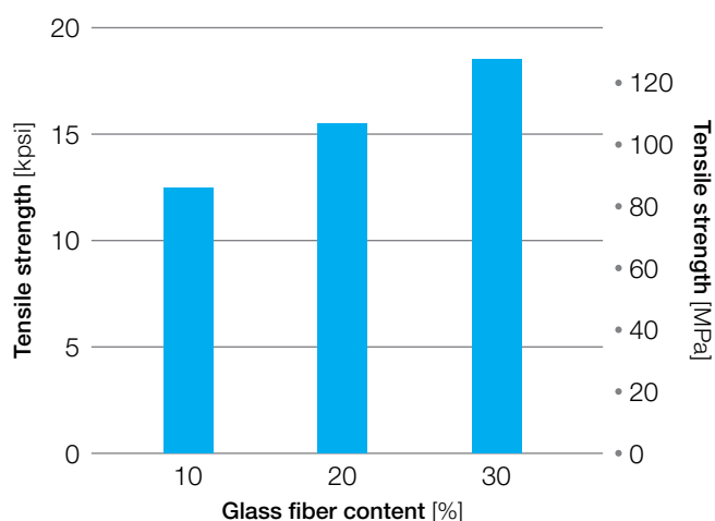
Figure 14: Tensile strength of glass-filled Veradel® PESU
