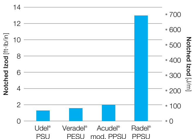
Figure 23: Notched Izod of neat resins
