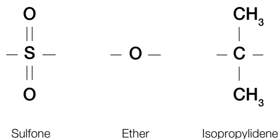
Figure 2: Bridging moieties
