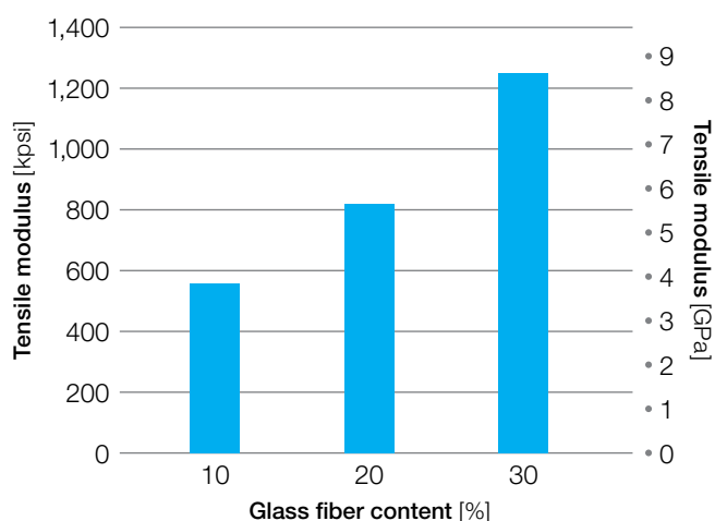
Figure 15: Tensile modulus of glass-filled Veradel® PESU
