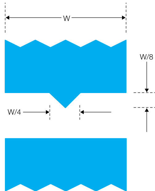
Figure 65: Energy director design
