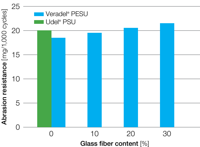
Figure 26: Abrasion resistance
