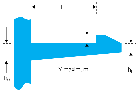
Figure 73: Snap-fit design using tapered beam
