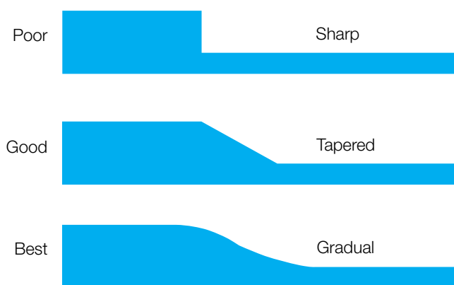
Figure 48: Wall thickness transition
