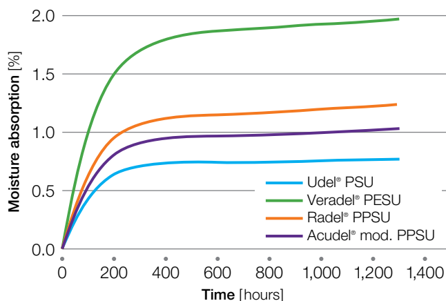
Figure 44: Water absorption by immersion at 23 °C (77 °F)
