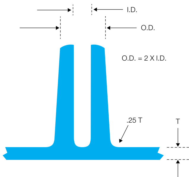
Figure 51: Boss design general guidelines
