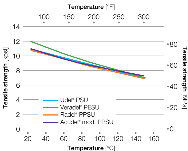
Figure 34: Tensile strength vs. temperature of neat resins
