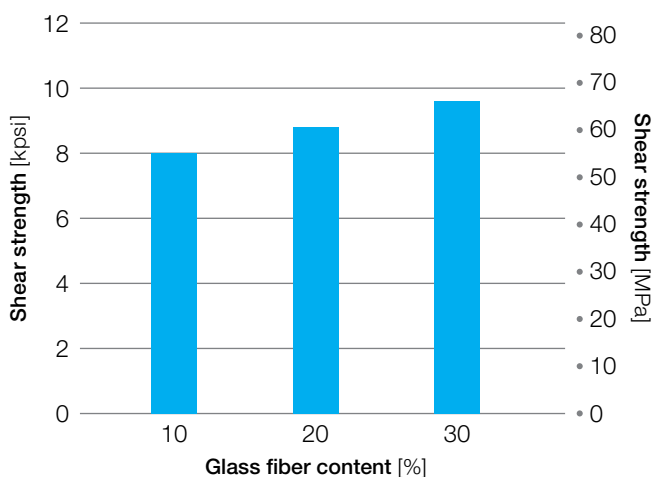
Figure 21: Shear strength of glass-filled Veradel® PESU
