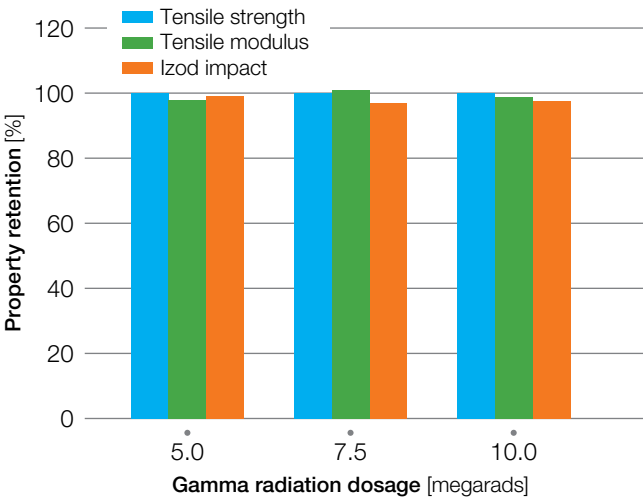
Figure 42: Radiation resistance of Radel® PPSU
