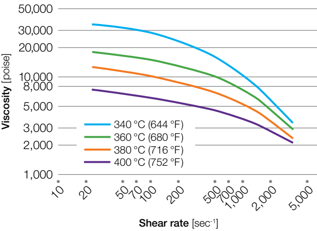
Figure 56: Rheology of Veradel® A-301 resin
