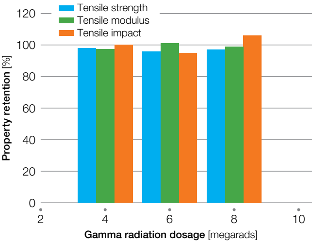
Figure 41: Radiation resistance of Veradel® PESU
