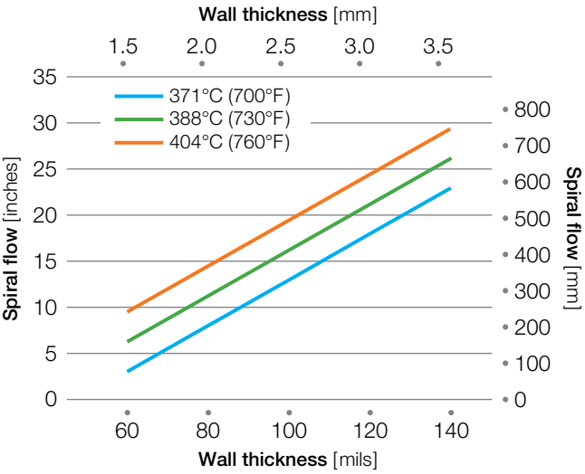
Figure 63: Spiral flow of Radel® R-5000 *
