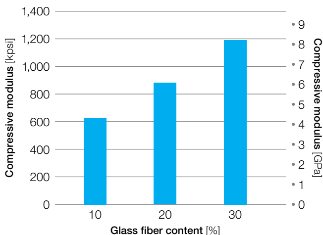
Figure 20: Compressive modulus of glass-filled Veradel® PESU
