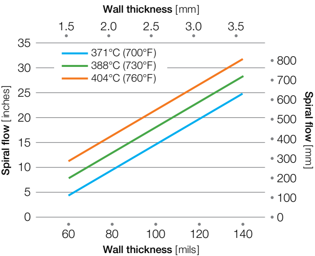
Figure 64: Spiral flow of Radel® R-5800 *
