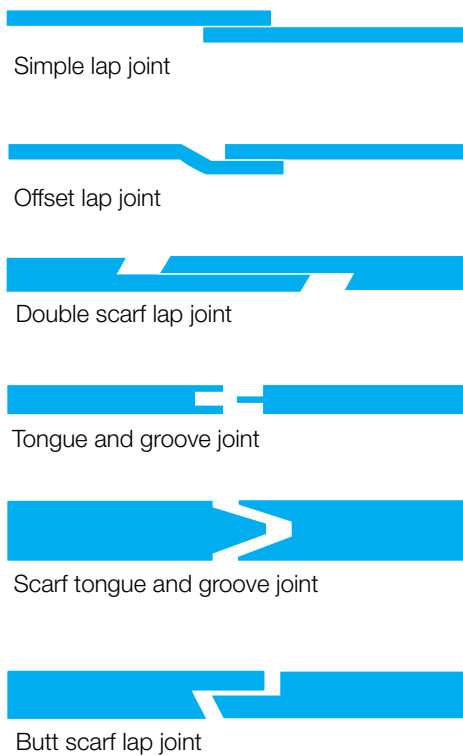
Figure 66: Joint designs for adhesive bonding
