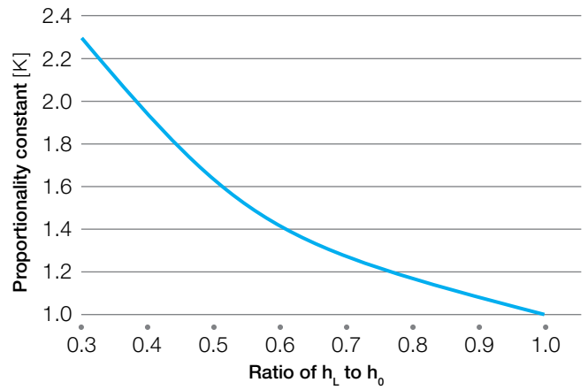
Figure 74: Proportionality constant (K) for tapered beam
