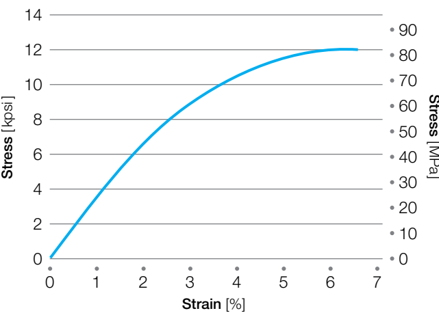
Figure 10: Radel® R-5000 stress-strain curve to yield
