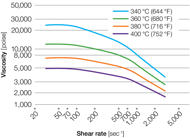
Figure 59: Rheology of Radel® R-5800 resin
