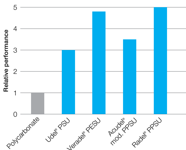
Figure 3: Relative thermal capability of sulfone polymers
