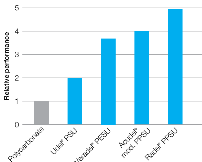
Figure 5: Chemical resistance of sulfone polymers
