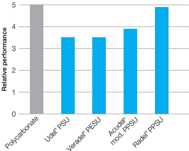
Figure 6: Impact resistance of sulfone polymers
